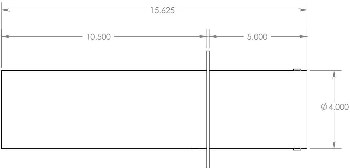
Side View
